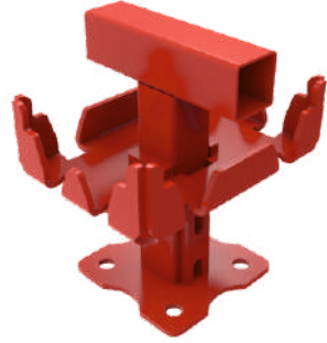
Slabmax Başlık Re-Shoring Slabmax Head Re-Shoring
